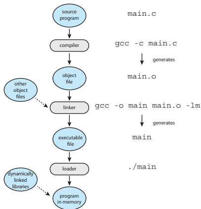
Figure: The role of the linker and loader. 4
